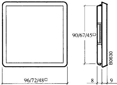
Cut-out cover
