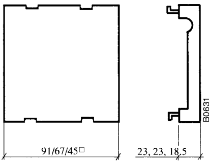
Protection cover
